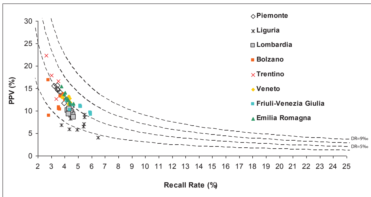
Figure 4S Recall rate (RR) versus positive predictive value (PPV); detection rate (DR) shown as isobars. Subsequent rounds. Northern Regions.
